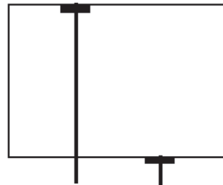
D.--Interval Biozone (based on highest occurrences).
