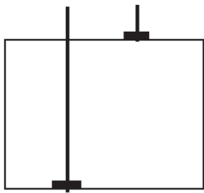
C.--Interval Biozone (based on lowest occurrences).
